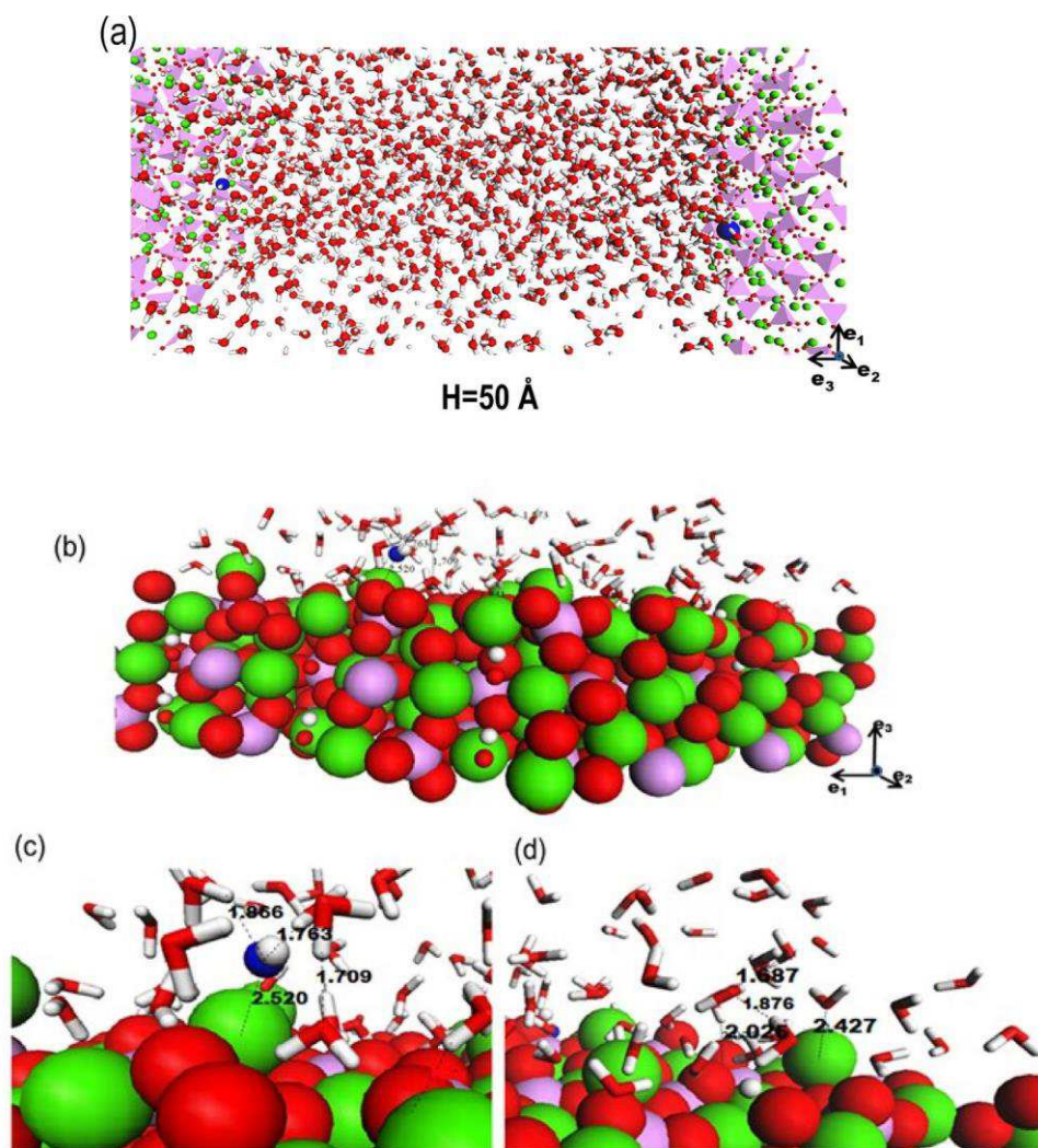
Fig. 3. Hydroxyl ions in HAP-Water system (Ca-green, \text{PO}_4^{3-} -pink, O-red, H-white and hydroxyl O-blue): (a) Molecular arrangement of water molecules and \text{OH}^- ions in a 50 Å HAP nanopore; (b) Interaction of \text{OH}^- ions with HAP-water layers; (c) and (d) shows the close views of H-bonds (distances are in Å) for \text{OH}^- -water and water-water, respectively, at the vicinity of HAP interface. (For interpretation of the references to colour in this figure legend, the reader is referred to the web version of this article.)
