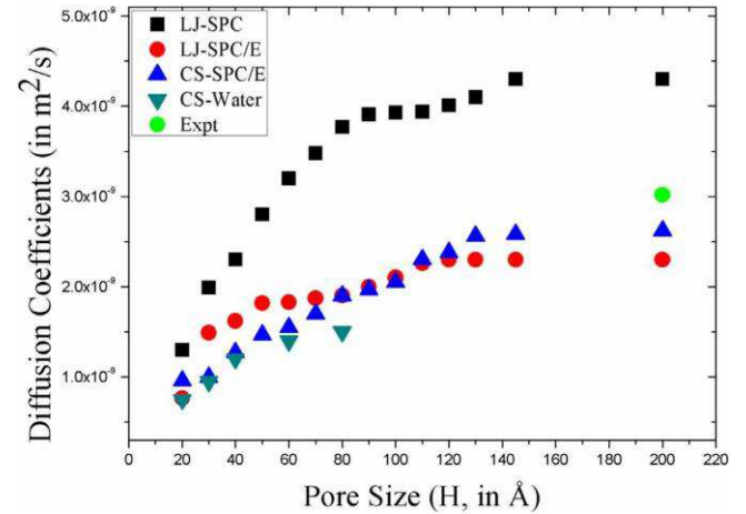
Fig. 2. Self-diffusion coefficients of water molecules calculated at 310 K for various pore sizes ( H = 20 to 200 Å) with different potentials models: LJ-SPC, LJ-SPC/E, CS-SPC/E, CS-water. The experimental diffusion coefficient is also presented.
