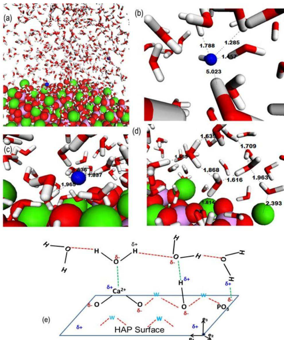
Fig. 4. Unusual hydroxyl ion diffusion in HAP-Water system (Ca-green, \text{PO}_4^{3-} -pink, O-red, H-white and hydroxyl O-blue): (a) Molecular arrangement of water molecules and \text{OH}^- ions in a 70 Å HAP pore; (b) and (c) Interactions of \text{OH}^- ion with water molecules near and far away from the HAP surface respectively; (d) H-bonded network between water molecules and \text{Ca}^{2+} -water interactions (Distances are in Å). (e) Schematic representation of HAP and water adsorption sites through H-bonding at interface. (For interpretation of the references to colour in this figure legend, the reader is referred to the web version of this article.)
