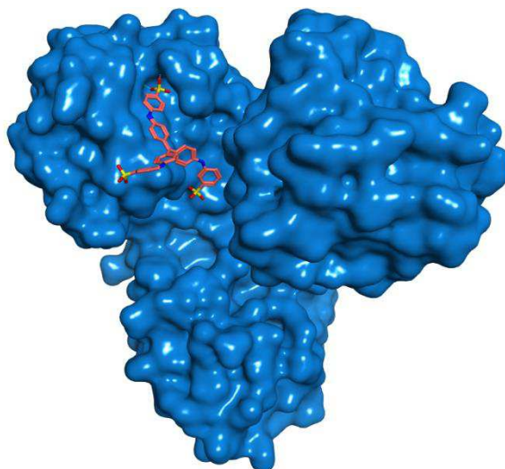
Figure 1: Crystal structure of 1 in complex with HCV NS3 helicase (PDB ID 1ZJO).
