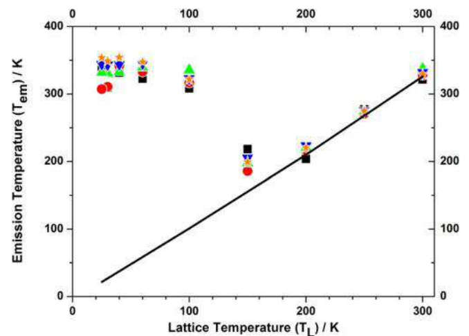
FIG. 2. Emission temperature ( T_{em} ) at fixed modal gains of 8 \text{cm}^{-1} (squares), 10 \text{cm}^{-1} (circles), 12 \text{cm}^{-1} (Up triangles), 16 \text{cm}^{-1} (down triangles), and 20 \text{cm}^{-1} (stars) plotted against lattice temperature ( T_L ) for the undoped sample. Also plotted is T_{em} calculated from the Fermi-Dirac model of the QD ensemble including HB (solid black line).
