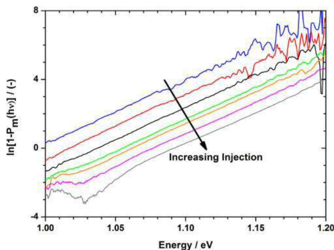
FIG. 1. Logarithmic plots of [1-P(h\nu)] versus photon energy for the undoped sample at measured at 300 K for current densities of 50 \text{Acm}^{-2} , 83.3 \text{Acm}^{-2} , 133.3 \text{Acm}^{-2} , 200 \text{Acm}^{-2} , 233.3 \text{Acm}^{-2} , 333.3 \text{Acm}^{-2} , 466.7 \text{Acm}^{-2} .
