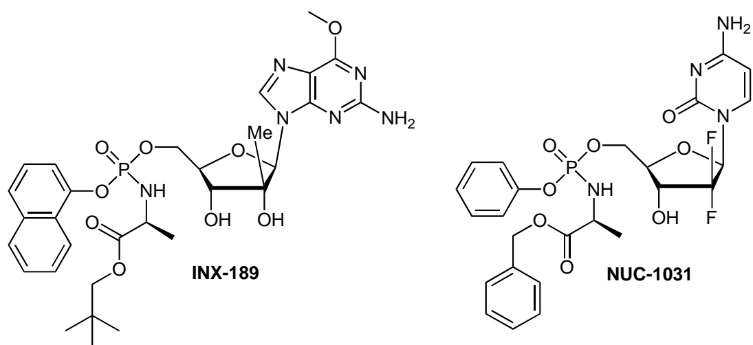
Figure 1. Chemical structures of ProTides INX-189 and NUC-1031.
