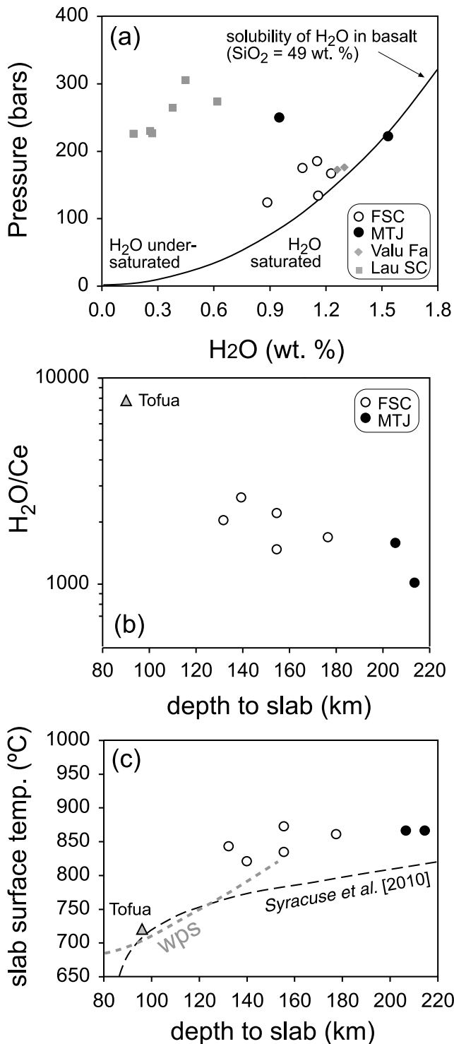
Figure 5. (a) H 2 O content versus pressure of recovery for glasses from Fonualei Spreading Center and Lau Basin lavas (data from Kent et al. [2002]) with MgO > 6 wt. % and for which U-series data are available. The curve is the H 2 O-saturated line for basaltic melts with 49 wt. % SiO 2 at 1150°C [after Newman and Lowenstern, 2002 ]. The implication is that the majority of samples would have been water-undersaturated at the depth of recovery and so the measured H 2 O contents provide a reasonable minimum estimate of primary magmatic H 2 O. (b) H 2 O/Ce versus depth to slab for the Fonualei Spreading Center samples and a Tofua basaltic-andesite as representative of the arc front [ Caulfield et al., 2012; Cooper et al., 2012 ]. (c) Slab surface temperature inferred from H 2 O/Ce after Plank et al. [2009] versus depth to slab. Note that any loss of H 2 O due to degassing would erroneously high temperatures. Also shown are the profile of slab surface temperatures from the D80 geophysical model of Syracuse et al. [2010] and the composite wet pelite solidus (wps) from Hermann and Rubatto [2009].
