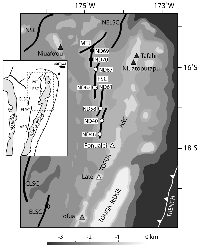
Figure 1. Map of the Fonualei Spreading Center showing the locations of samples analyzed in this study: Fonualei Spreading Center (FSC, unfilled circles); Mangatolu Triple Junction (MTJ, filled circles). Also included are the locations of Tofua arc islands: Tofua (shaded triangle); the FSC proximal islands of Late and Fonualei (unfilled triangles); and the northern islands of Niuatoputapu and Tafahi (filled triangles). Inset shows the location within the Tonga arc–Lau Basin system and the major tectonic elements therein (VFR – Valu Fa Ridge, ELSC – Eastern Lau Spreading Center, CLSC – Central Lau Spreading Center, NSC – Niuafu’ou Spreading Center, FSC – Fonualei Spreading Center, MTJ – Mangatolu Triple Junction). Shading and scale bar indicate bathymetry.
