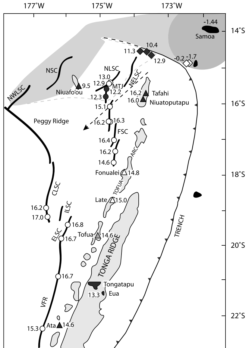
Figure 3. Map of the Tonga arc–Lau Basin system showing \epsilon\text{Hf} numbers for analyzed basalts and the inferred extent of influence from Samoan plume mantle (assuming \epsilon\text{Hf} < 13 ) that is inferred to influx into the back-arc through a tear in the subducting slab. The dark shaded zone indicates a minimum radius for the Samoan plume based on inclusion of the seamounts within it. The lighter shaded zone is the likely extent of Samoan influence, after interaction with shallow mantle flow, based on He isotope data [Turner and Hawkesworth, 1998; Lupton et al., 2009] while the dashed line indicates the possibly larger extent based on Pb [Regelous et al., 2008] and Hf isotope data (sources as for Figure 2). Abbreviations and symbols as in Figures 1 and 2. The new boninite and seamount data suggest that the tear in the slab ceases somewhere in the vicinity of the boninite localities. The arrow indicates the general direction of mantle flow, if the He, Nd and Hf isotope systems become modified by preconditioning (see text for explanation).
