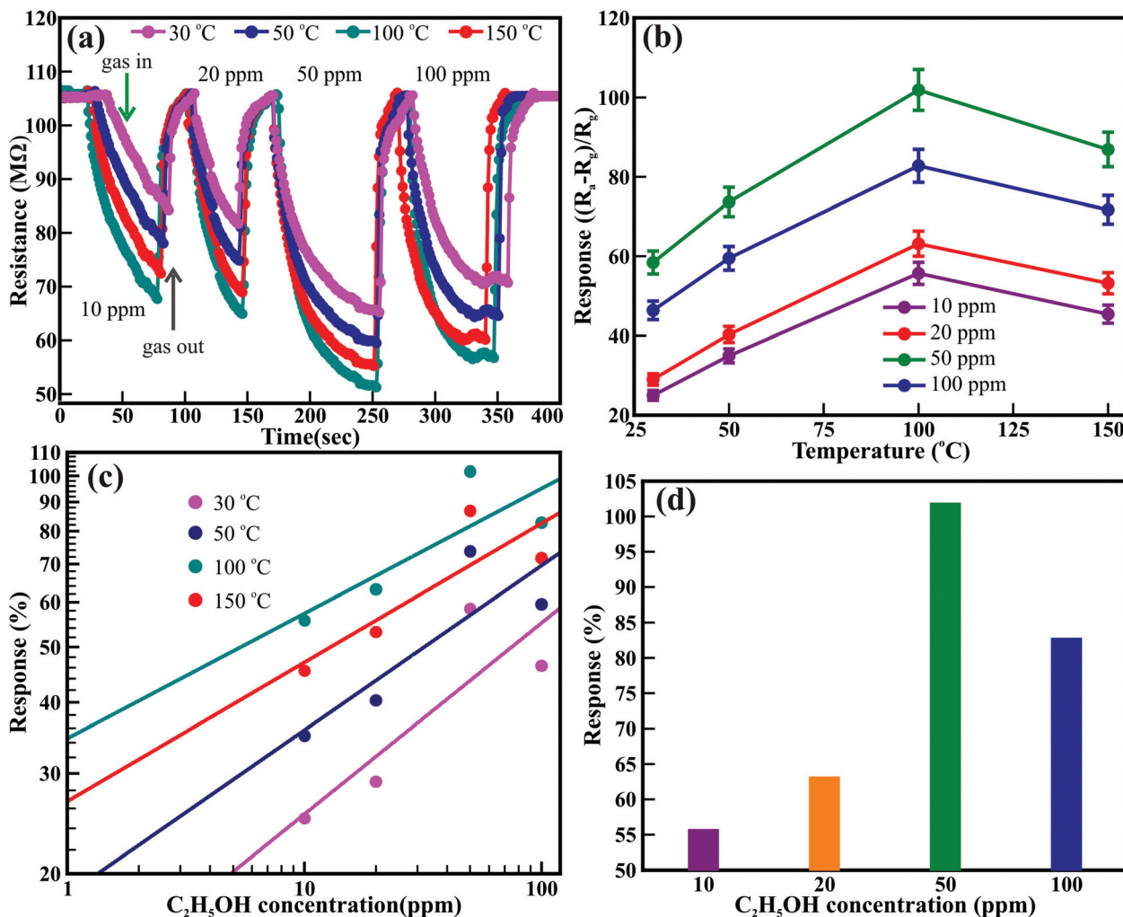
Fig. 4 (a) Time-dependent response–recovery behavior of ZnO nanowires with different concentrations of C_2H_5OH gas at various operating temperatures ( i.e. , 30 °C, 50 °C, 100 °C and 150 °C). (b) Temperature-dependent response behavior of ZnO nanowires with different concentrations of C_2H_5OH gas. (c) C_2H_5OH concentration-dependent response behavior of ZnO nanowires at different operating temperatures. (d) The optimum sensing response of the ZnO nanowires sensor as a function of C_2H_5OH concentration at the operating temperature of 100 °C.
