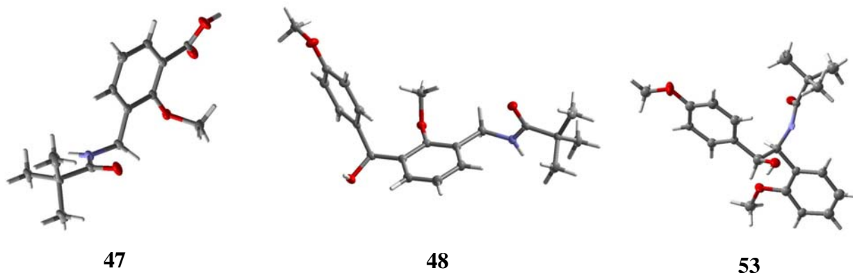
Figure 5. X-ray crystal structures of compounds 47 , 48 and 53 .
