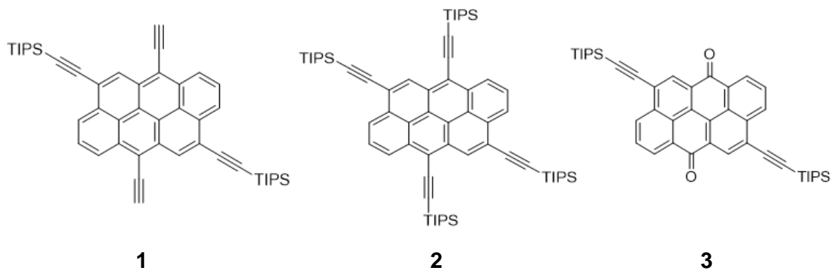
Scheme 1. The anthanthrene ( 1 and 2 ) and anthanthrone ( 3 ) derivatives studied here.
