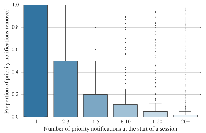
Figure 8: The proportion of removed priority notifications, grouped by the number of dismissible priority notifications
