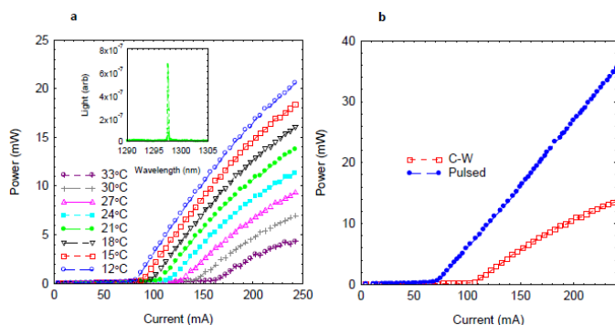
Fig. 2 (a) Power-current characteristics vs. temperature for a 10 \mu\text{m} \times 3 \text{mm} laser operating CW. Inset: shows lasing wavelength at 21°C and at 10% above threshold current. (b) Power-current curves for 10 \mu\text{m} \times 3 \text{mm} laser operated pulsed (solid symbols) and CW (open symbols).
