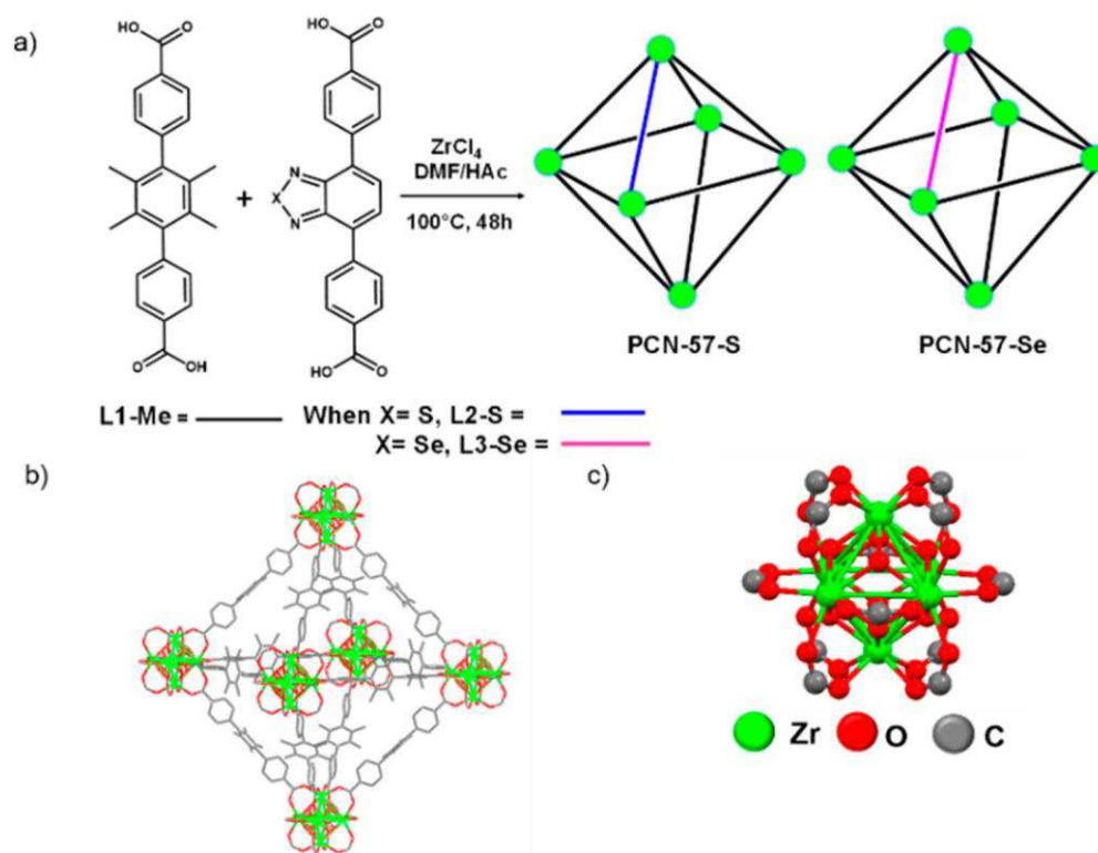
Figure 1. (a) Schematic representation of the synthesis of PCN-57-S and PCN-57-Se using a mixed ligand approach. (b) Structure of PCN-57. (c) Structure of the Zr 6 node of PCN-57.
