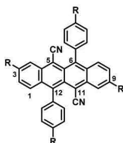
Tet , R = H, Me, TMS, F
