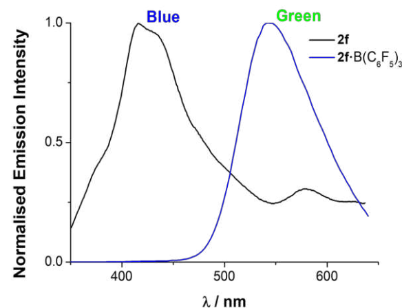
Figure 7. Solid-state film fluorescence spectra of 2f and 2f · \text{B}(\text{C}_6\text{F}_5)_3 ( \lambda_{\text{ex}} = 330 nm).
