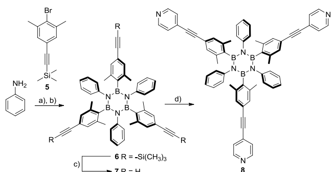
Scheme 2. Synthesis of BNAPy 8 : a) \text{BCl}_3 , toluene, reflux, 18 h; b) 5 , t\text{-BuLi} , THF, -84^\circ\text{C} , 16 h, 71%; c) TBAF, THF, 0^\circ\text{C} , 2 h, 94%; d) 4-iodo-pyridine, [\text{PdCl}_2(\text{PPh}_3)_2] , \text{PPh}_3 , \text{CuI} , \text{NEt}_3 , 75^\circ\text{C} , 17 h, 70%.
