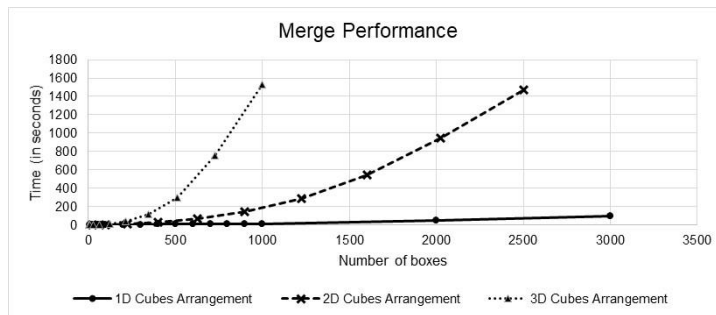
Fig. 8: The merge operation’s performance given different numbers of cubes in three arrangements.
