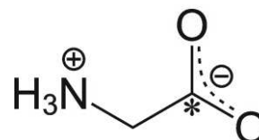
Scheme 1. Molecular structure of glycine (the asterisk indicates the labelled ^{13}\text{C} site in 1\text{-}^{13}\text{C} -glycine).
