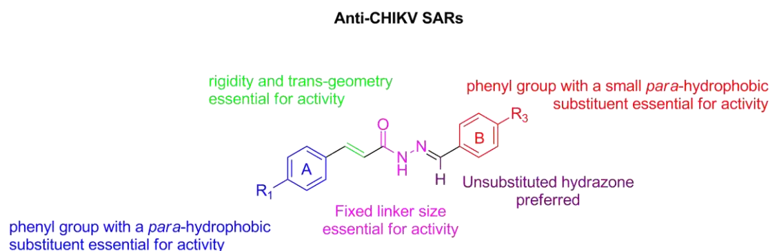
Figure 3. Summary of the antiviral structure-activity relationships obtained with this work for the antiviral scaffold of 1 and 2 .
