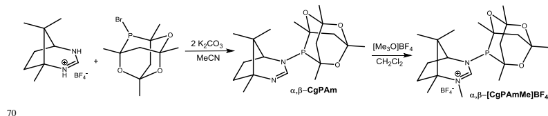
Scheme 1. Synthesis of \alpha,\beta -CgPAm and [\alpha,\beta -CgPAmMe]BF 4 .
