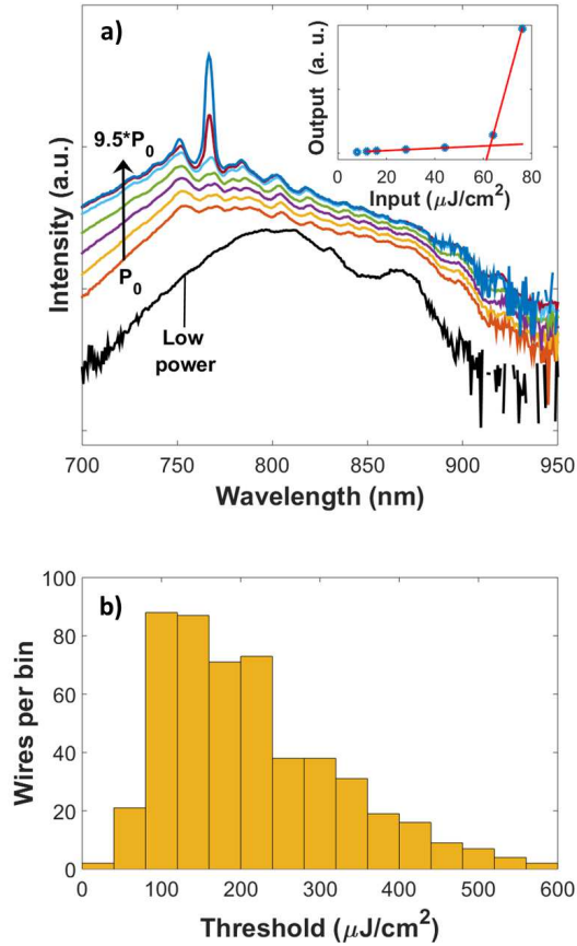
Figure 2: a) Power dependent PL spectra of a selected low-threshold NW laser, where the lowest excitation fluence is indicated as P_0 = 8 \mu\text{Jcm}^{-2} per pulse. The lowest curve (in black) shows the PL spectrum measured under low-power continuous excitation for the same wire. Inset: LILO curve. An abrupt change in slope is observed at 63 \mu\text{Jcm}^{-2} , associated with the transition to lasing behavior. b) A histogram of threshold pump values calculated for 579 lasing NWs.
