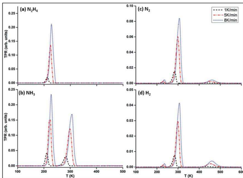
Fig. 3 Simulated TPR curves for N_2H_4 , NH_3 , N_2 and H_2 desorption from the Cu(111) surface, starting from an initial N_2H_4 coverage of 1 ML (full coverage) at a reaction time of 1 s for different heating rates.
