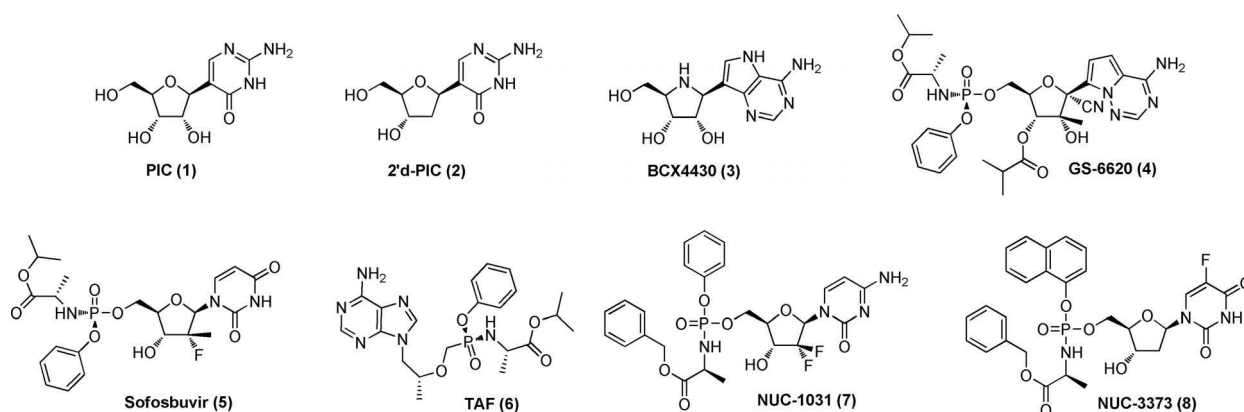
Figure 1. Structures of pseudoisocytidine (PIC, 1), 2'-deoxypseudoisocytidine (2'-d-PIC, 2), BCX4430 (3), GS-6620 (4), sofosbuvir (5), tenofovir alafenamide (TAF, 6), NUC-1031 (7), and NUC-3373 (8).
